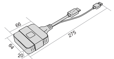
IQShare Button: 64mm*66mm*20mm(without wire) 64mm*275mm*20mm(with wire)
